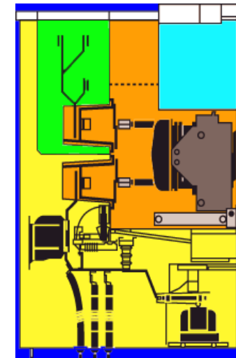
Metal-Clad Switchgear
