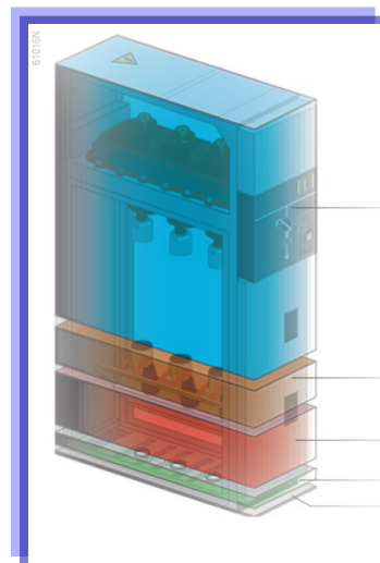
Compartmented Switchgear
