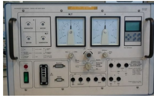
Control Unit Servo Brake 300W. "ELWE"
