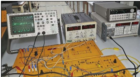
Figure 5.38: De Lorenzo Equipment for Frequency Modulation (FM) and Demodulation set using various techniques; measurements in HP Oscilloscope.
