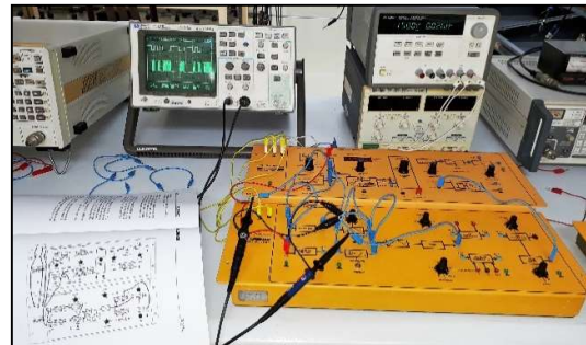
Figure 5.38: De Lorenzo Equipment for Frequency Modulation (FM) and Demodulation set using various techniques; measurements in HP Oscilloscope.
