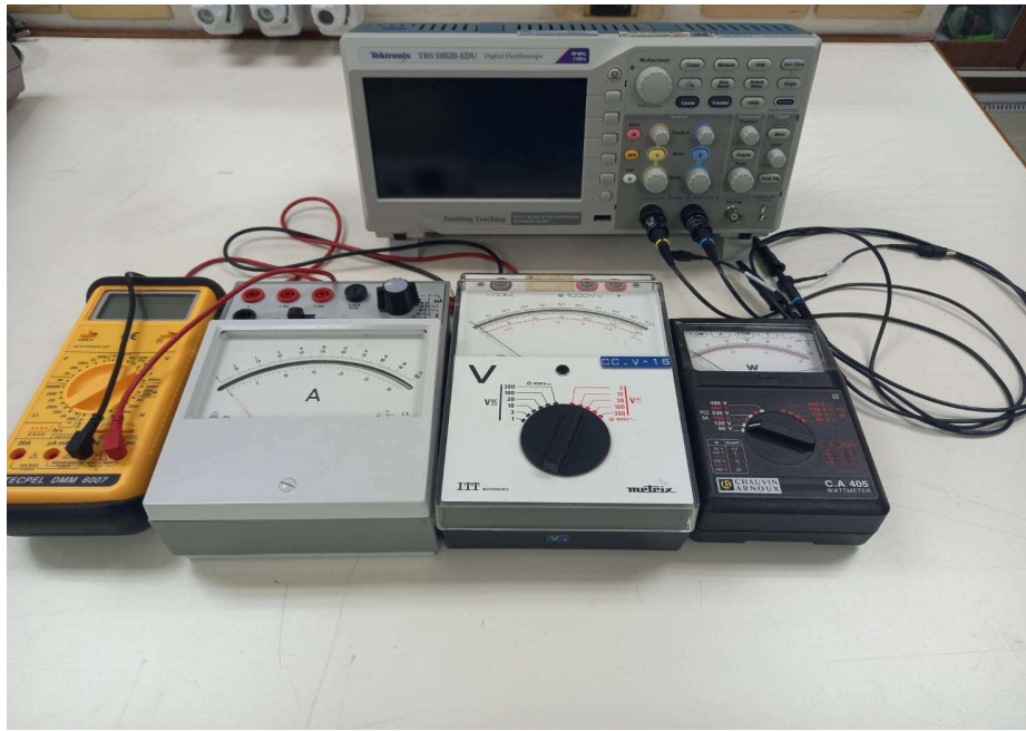
Figure 5.2: Digital Multi-Meter (DMM), Ammeter, Voltmeter and Wattmeter (from left to right)
